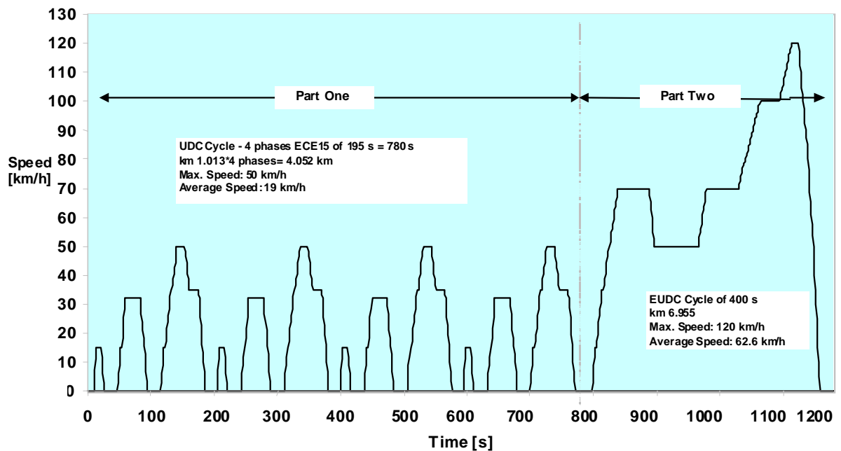
Figure 3.1 NEDC Cycle
