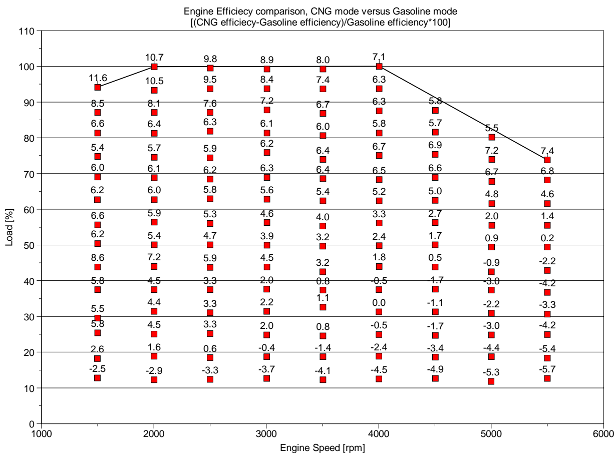
Figure 4.1.3 Efficiency difference between Gasoline and CNG
