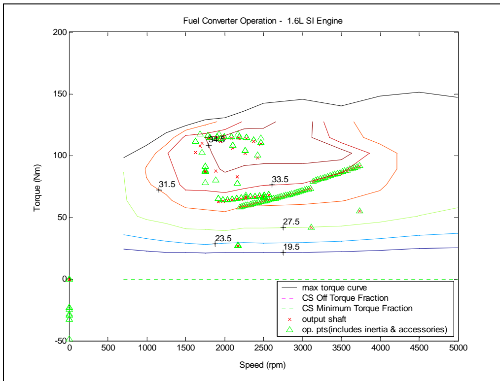
Figure 5.2.5-1 1.6 l engine operating points during the NEDC
