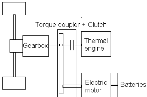
Figure 5.2 Simulated hybrid configuration
