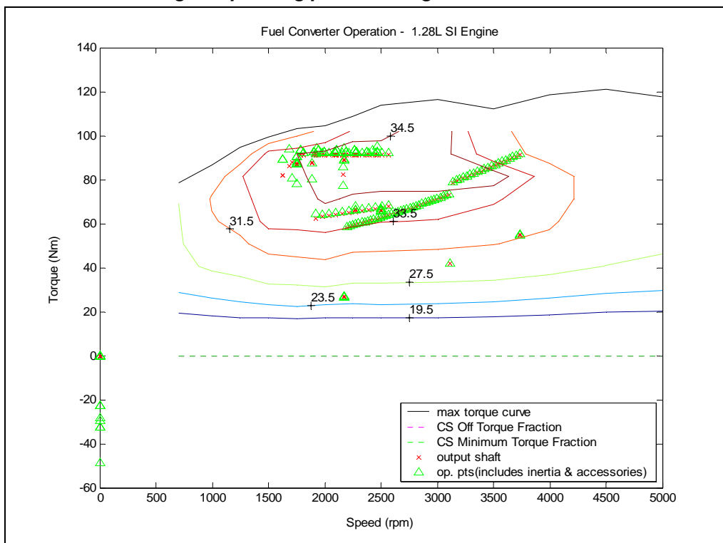
Figure 5.2.5-2 1.28 l engine operating points during the NEDC
